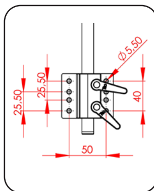
Mounting Plate Measurments In mm
